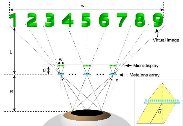
Fig. 4. Metalens array with a freeform phase response profile for FOV expansion: a linear phase term dependent on incident angle and a quadratic term.
