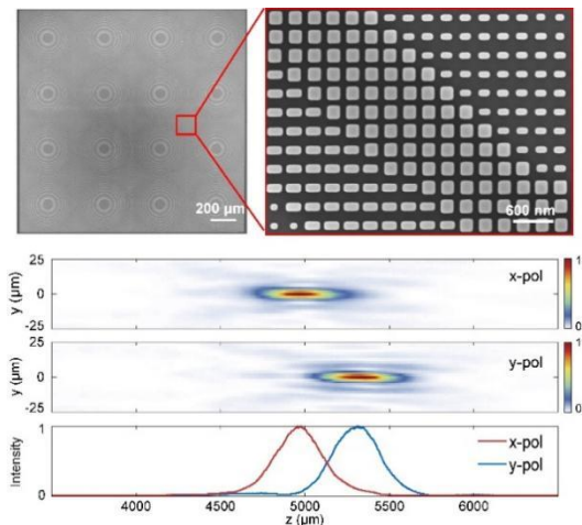
Fig. 2. The PM metalens derive (upper) and the focal length test for x- and y- linearly polarized light.
