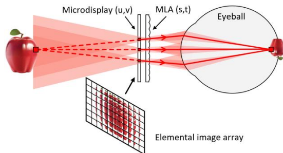
Fig. 1. General architecture of near-eye light field displays
